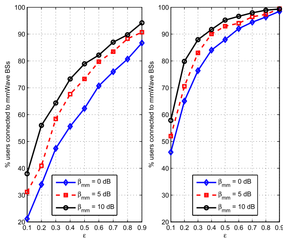
Fig. 10: User association for different values of \epsilon with v_1 + v_2 = 20 BSs/km 2 for \alpha = 3 (left) and \alpha = 4 (right).
