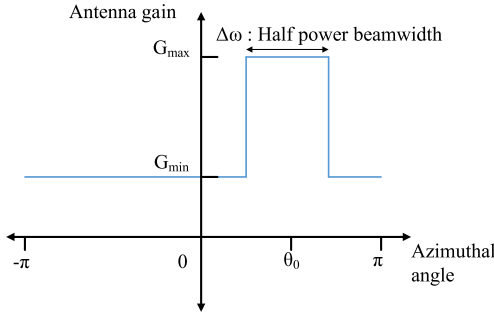
Fig. 2: Antenna Sectoring
