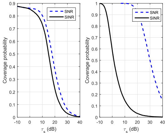
Fig. 3: Comparison of SNR and SINR in mmWave (left) and UHF (right) networks with v_1 = v_2 = 15 BSs/km 2 .
