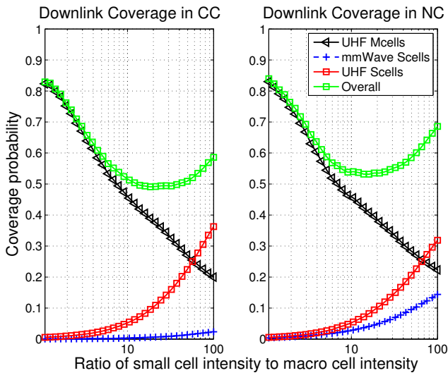
Fig. 4: Downlink coverage in NC and CC.
