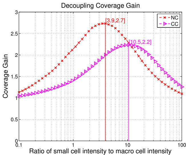
Fig. 2: Coverage gain for different small cell densities
